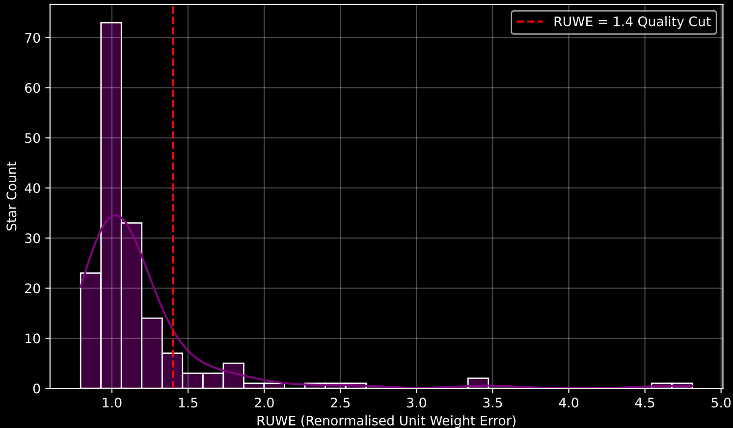
GAPOGEE DR17 Field [169+53_MGA] RUWE Distribution (n= 170)
