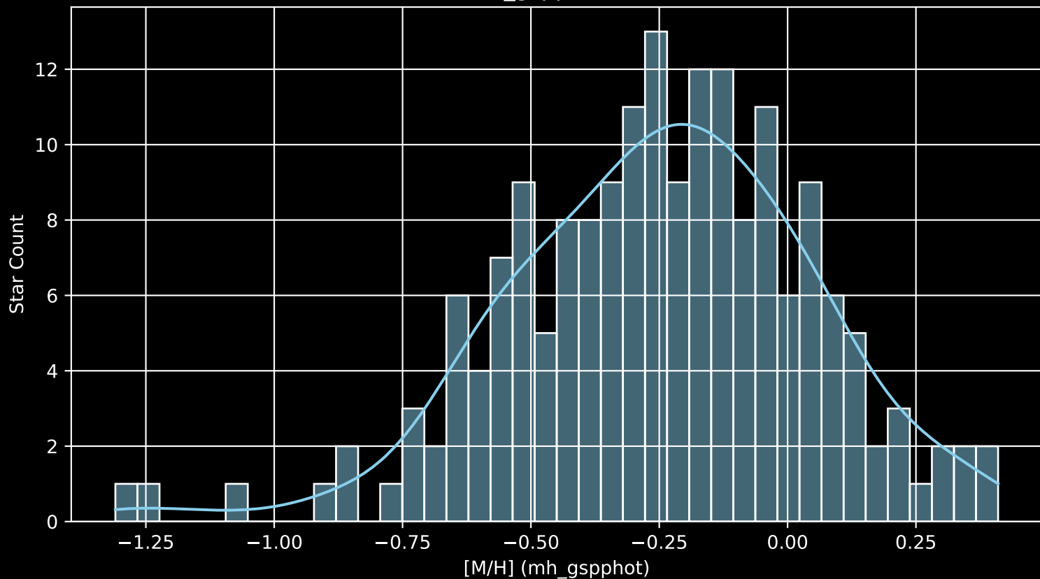
APOGEE DR17 Field: [169+53_MGA [M/H] (mh_gspphot) (n= 182)
