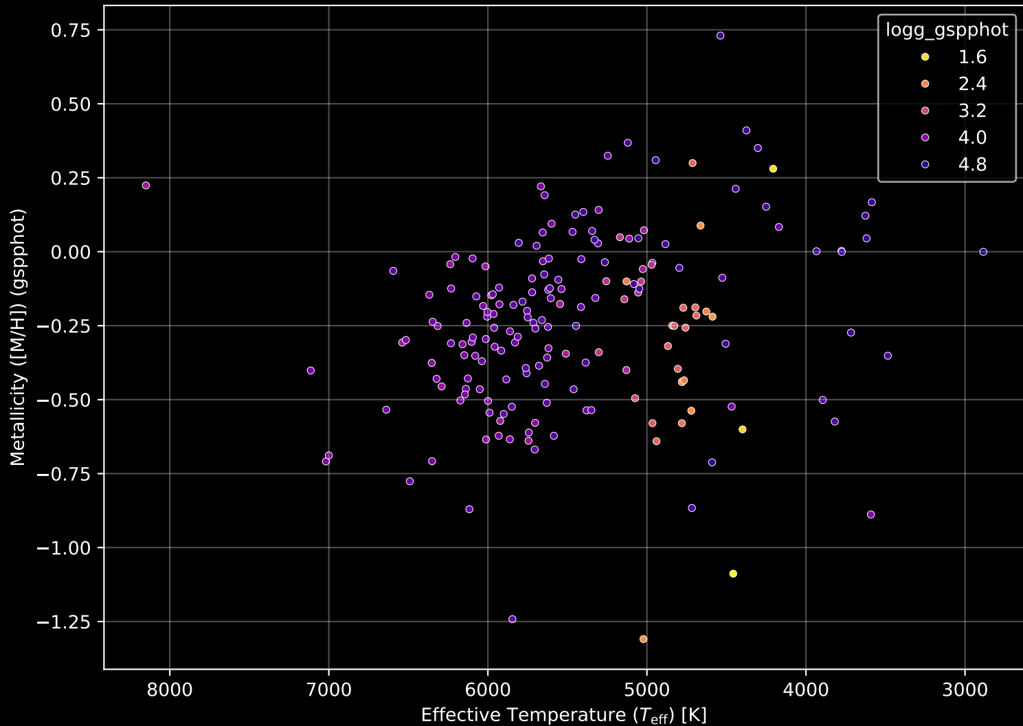
APOGEE DR17 Field: [169+53_MGA] Stellar Population Parameters (n= 183)
