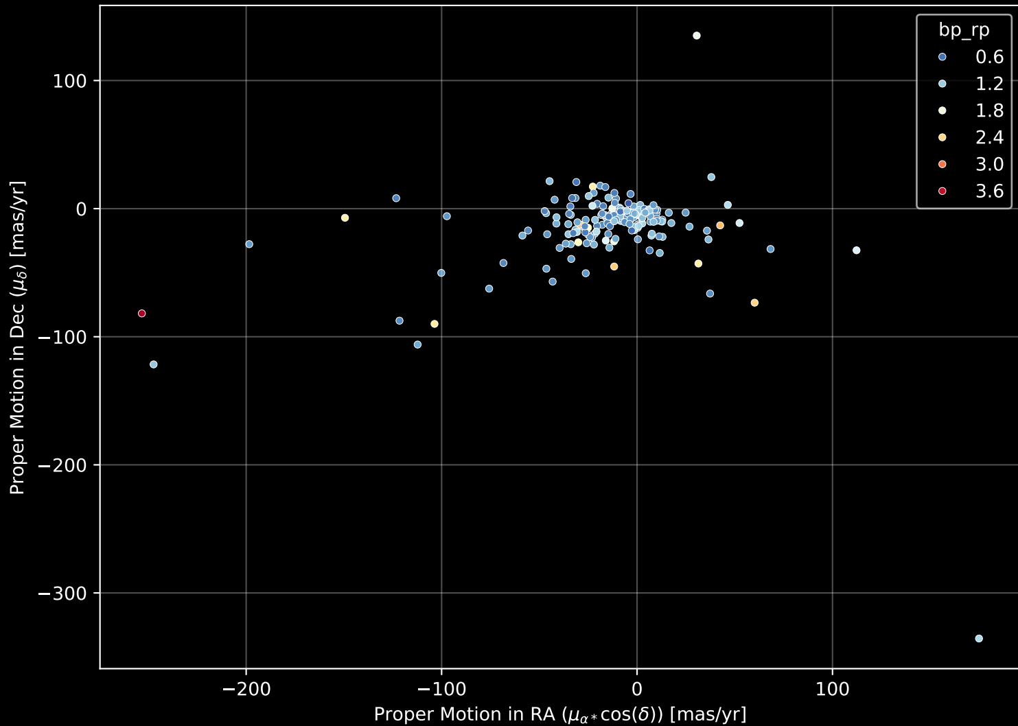
APOGEE DR17 Field: [169+53_MGA] Proper Motion Diagram (n= 183)
