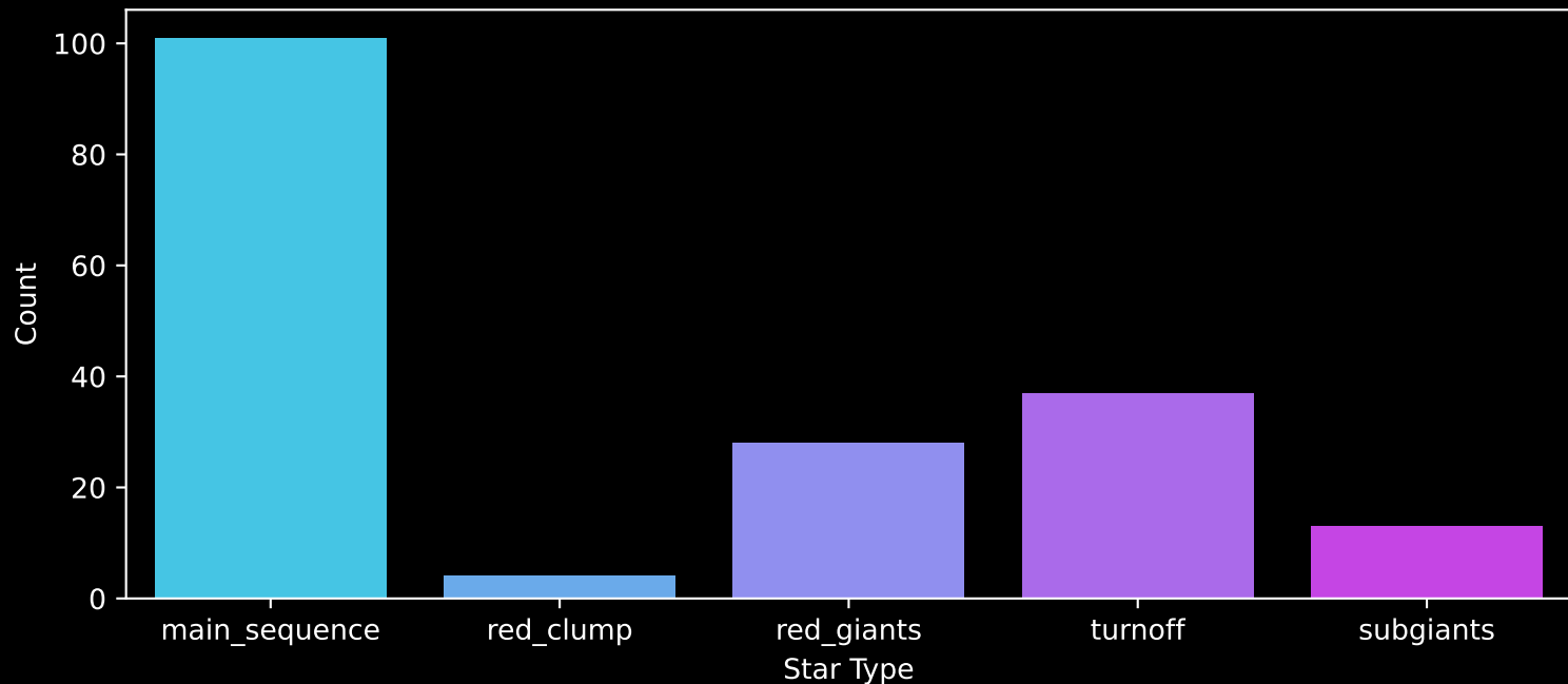
APOGEE DR17 Field: [169+53_MGA] Count plot of Star Type
