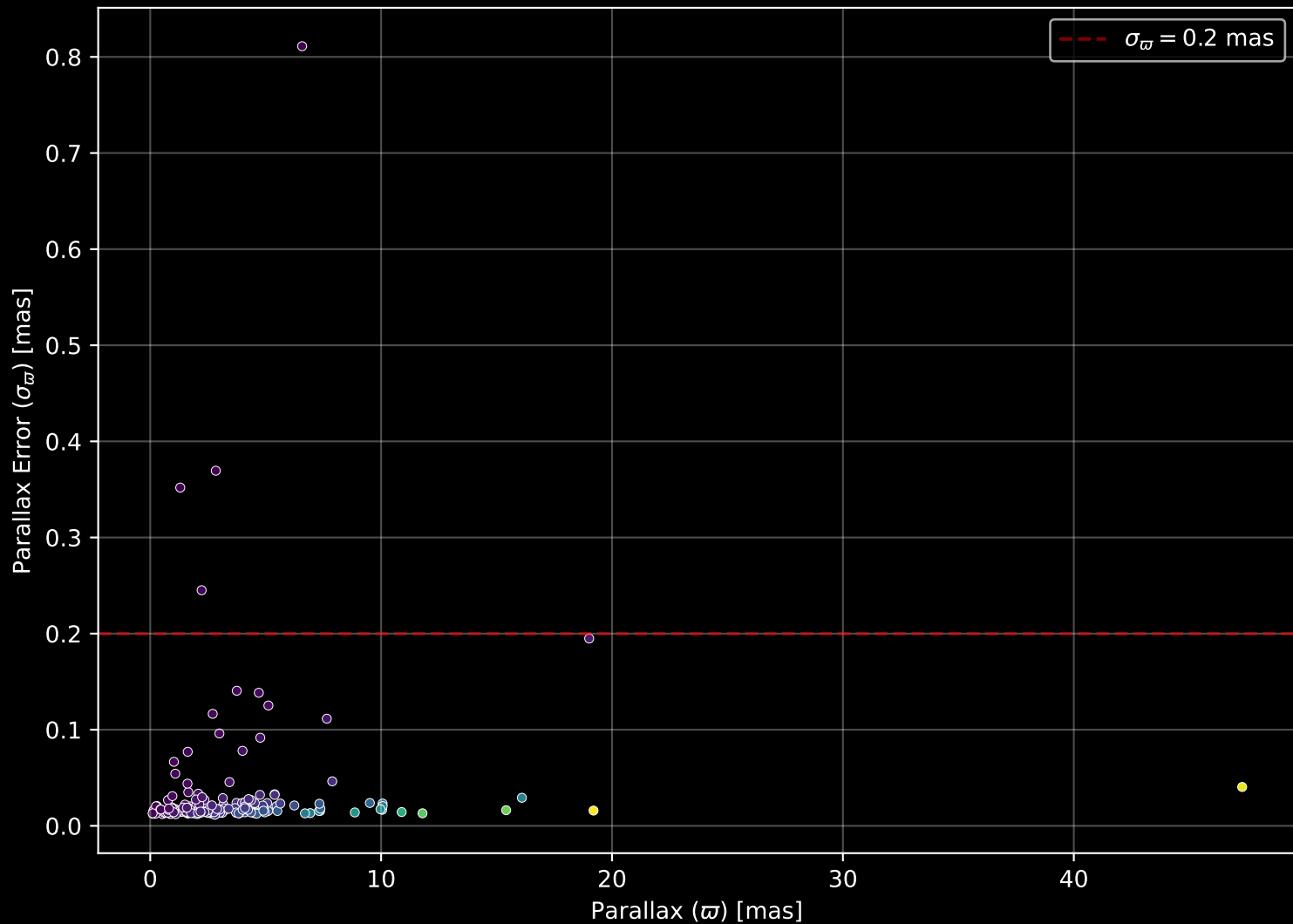
APOGEE DR17 Field: [169+53_MGA] Parallax Quality (n= 183)
